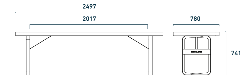
Vista Frontal
